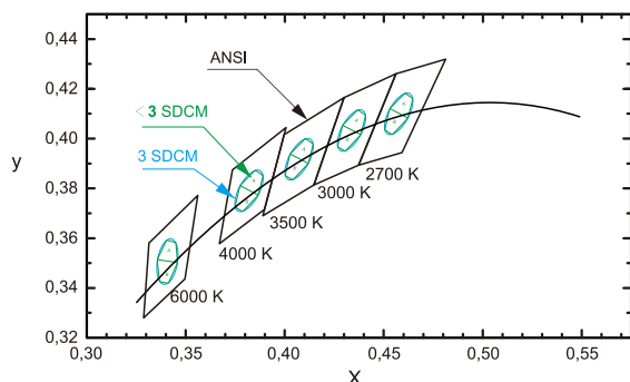
Narrow spectrum
