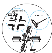
Mechanical connection
