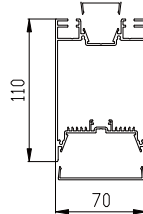
2. Extrusion lamp body & PC diffuser.
