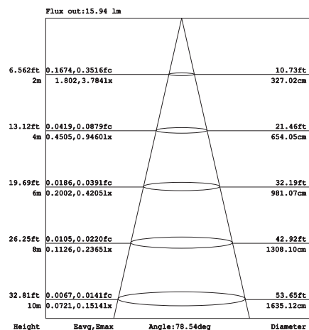
Effective Average Illuminance
