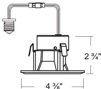
Square Baffle Trim
