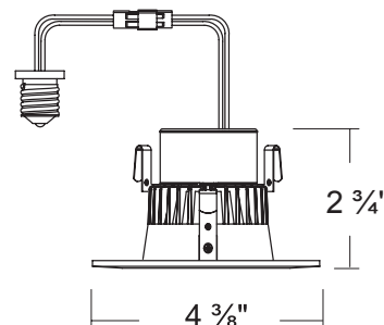
Circular Baffle Trim
