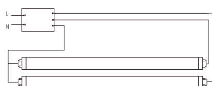
Electronic ballast
